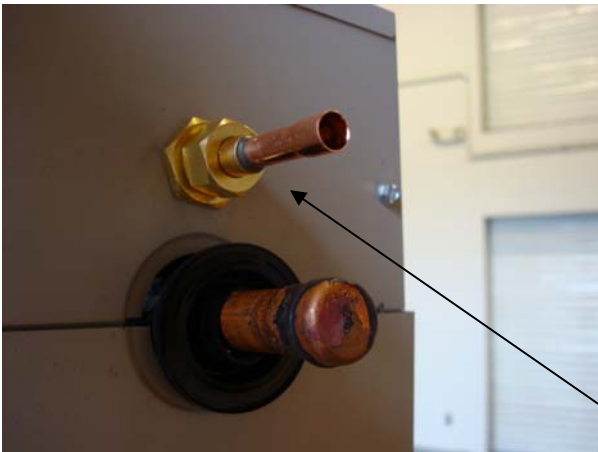
Liquid line brazing stub (664378) with nut (664387)
